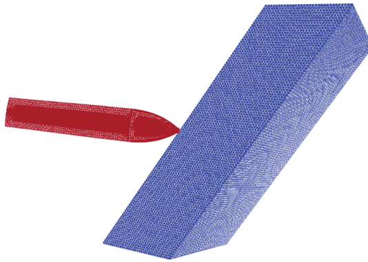
Figure 8: MPM models for simulation of oblique penetration.
